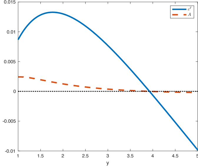
Figure 3: The blue solid line corresponds to \hat{c}^T whereas the orange dashed line represents the tax A on information acquisition. The two curves switch signs for the same value of y . The parameter values used for this simulation are: \lambda = \beta = \tau_e = \tau_\eta = \tau_\theta = 1 , \tau_u = 30 , and 1 \leq y \leq 5 .
